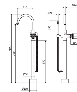
art. P1-KM04 - .. * Century Handle for mixer
