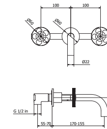
art. P1-BW50 - ..* 3 holes wall mounted basin mixer art. P1-KT04 - ..* Century Kit for 2 handle tap
