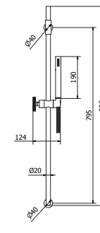
art. P1-KM02 - ..* Chicago Handle for mixer
